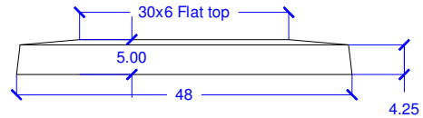
PC4824-1 not Square 1 mold
