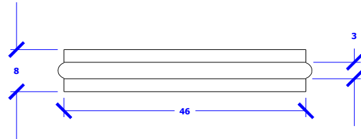
PC46 Bull Edge Adjustable to 46x46
